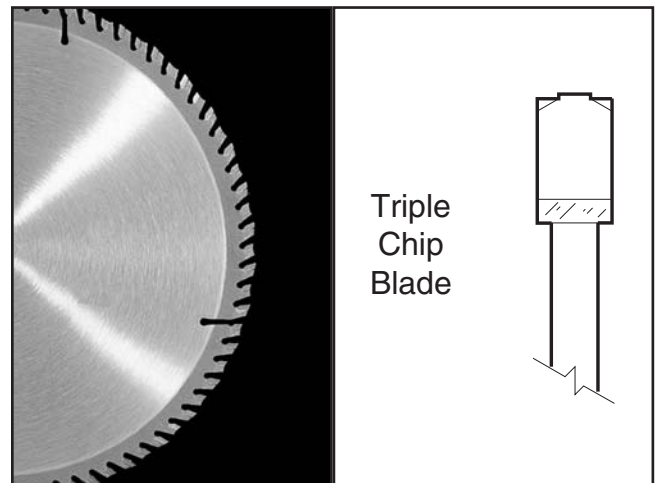
Figure 47. Laminate blade.
